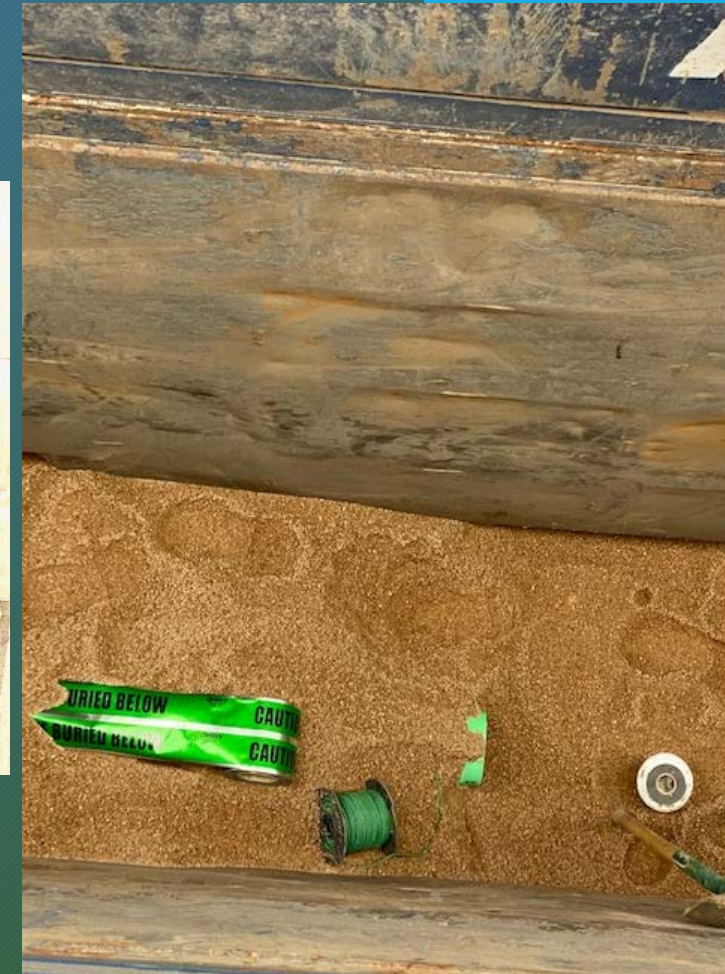
Trace Wire on Sewer Service
